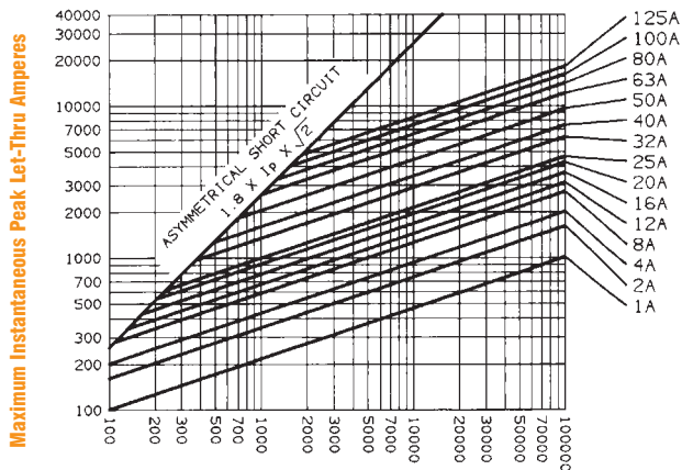
Available Current in RMS Symmetrical Amperes
