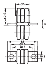
CP 2x36x27 - With built-in trip-indicator
