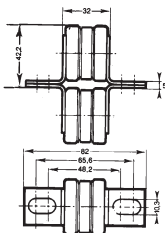
CP 2x36x27 - Without trip-indicator
