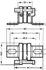
CP 36x27 - With separated trip-indicator
