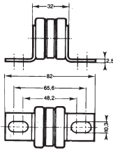
CP 36x27 - With built-in trip-indicator
