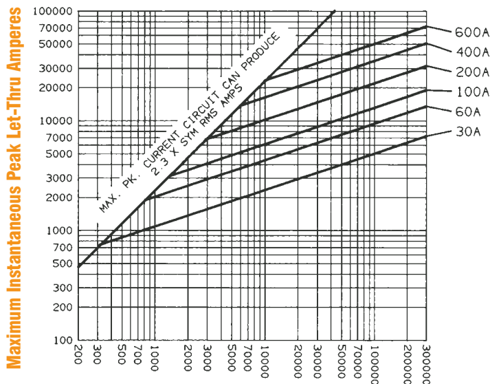
Peak Let-Thru Current Data – A6D30 to 600, 600 Volts AC
