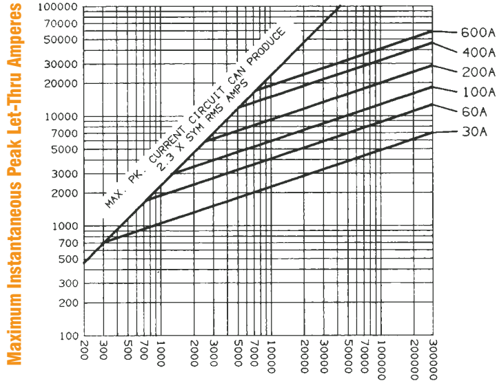
Peak Let-Thru Current Data – A2D30 to 600, 250 Volts AC
